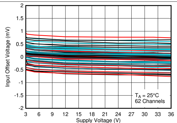
Figure 17. Input Offset Voltage vs. Supply Voltage at 25^\circ\text{C}
