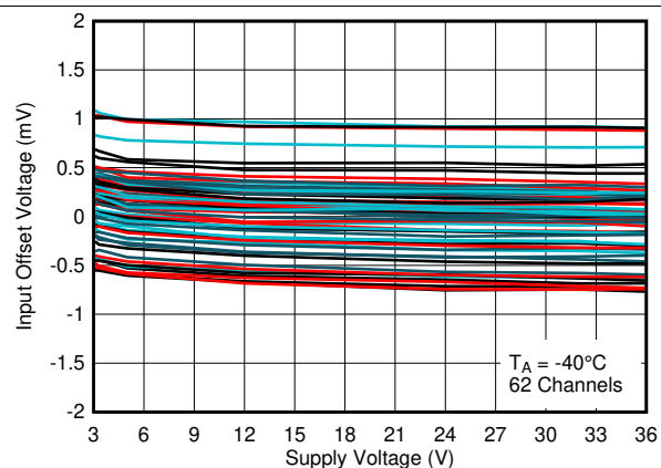
Figure 16. Input Offset Voltage vs. Supply Voltage at -40^\circ\text{C}
