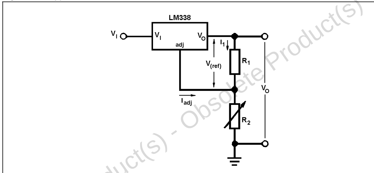
Figure 18. Application circuit
