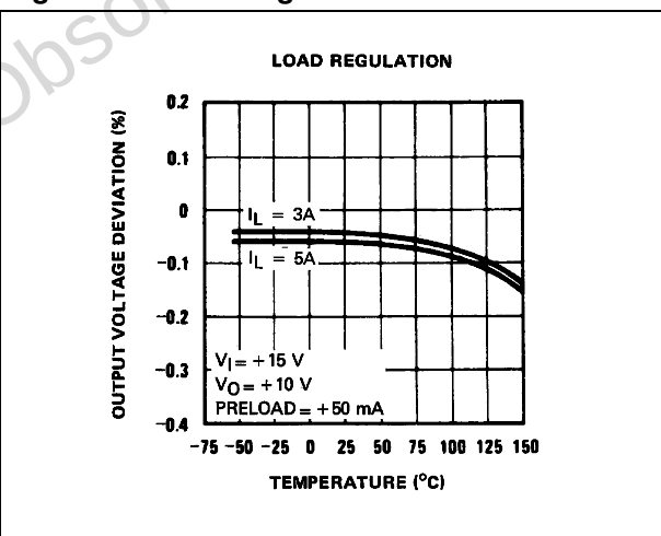
Figure 6. Load regulation
