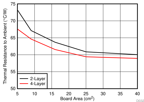
Figure 82. Package Thermal Resistance vs Board Copper Area
