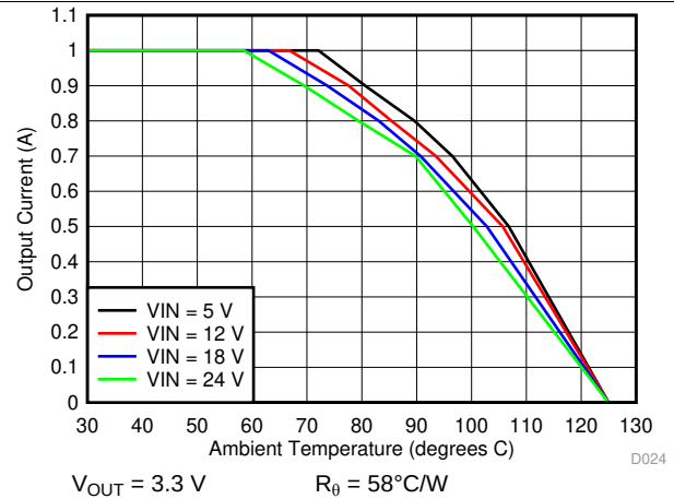
Figure 20. Ambient Temperature vs Output Current
