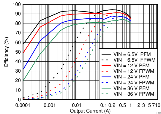
Figure 76. Efficiency for V_{OUT} = 5\text{ V}
