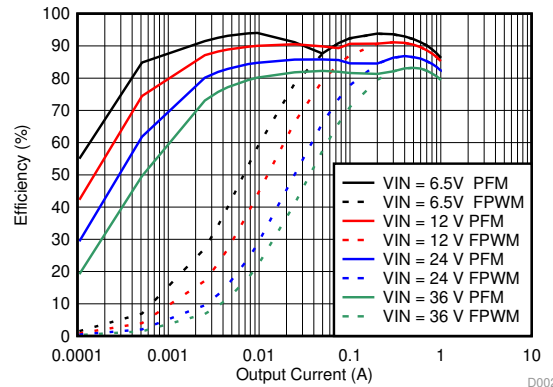
Figure 40. Efficiency
