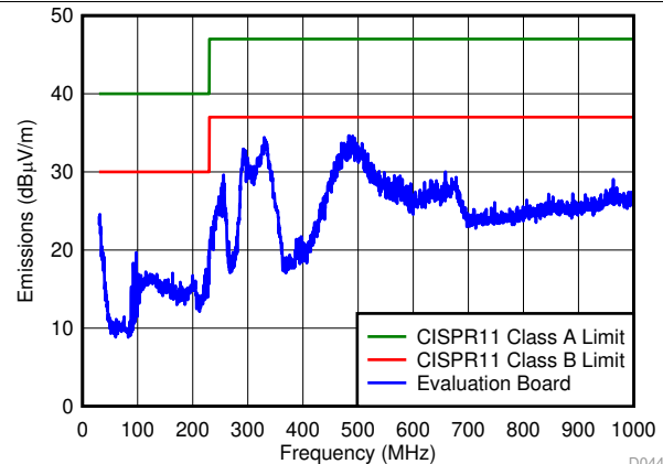
V_{IN} = 24\text{ V} I_{OUT} = 1\text{ A} Default EVM BOM with GND Plane as Top Layer
