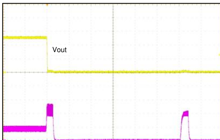
Figure 34. Hiccup Operation
