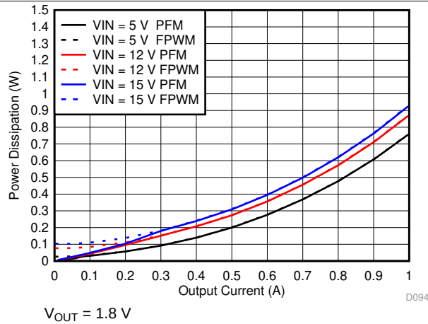
Figure 15. Power Dissipation
