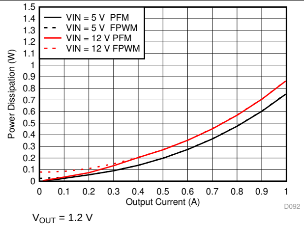
Figure 16. Power Dissipation
