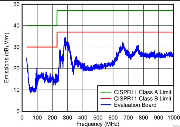
V_{IN} = 24\text{ V} I_{OUT} = 5\text{ A} Default EVM Layout with added 3 × 100pF 0603 C IN
