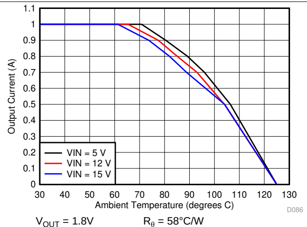
Figure 18. Ambient Temperature vs Output Current
