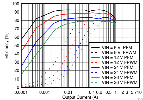
Figure 77. Efficiency for V_{OUT} = 3.3\text{ V}
