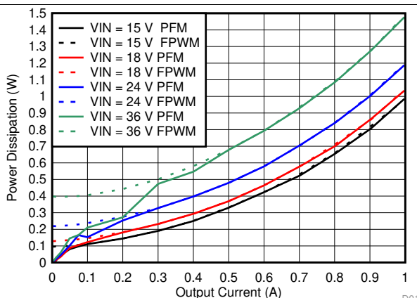
V_{OUT} = 12\text{ V}
