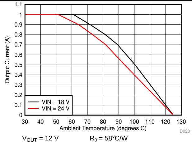
Figure 22. Ambient Temperature vs Output Current
