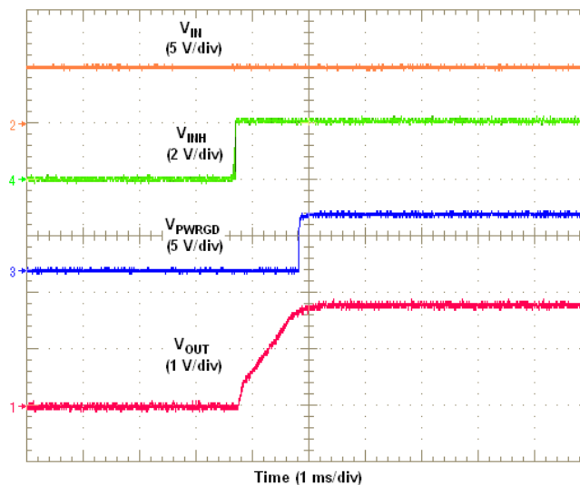
Figure 24. Inhibit Turn-On
