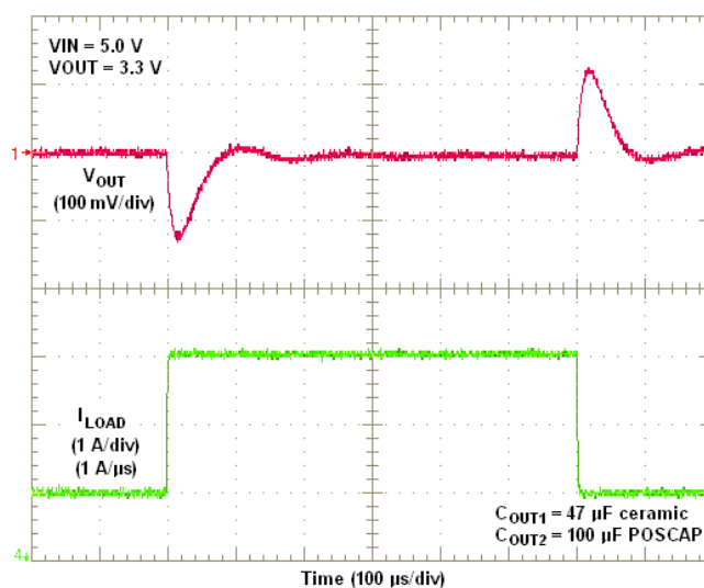
Figure 18. V_{IN} = 5\text{V} , V_{OUT} = 3.3\text{V} , 2A Load Step
