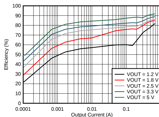
Efficiency for V_{IN} = 12 V
