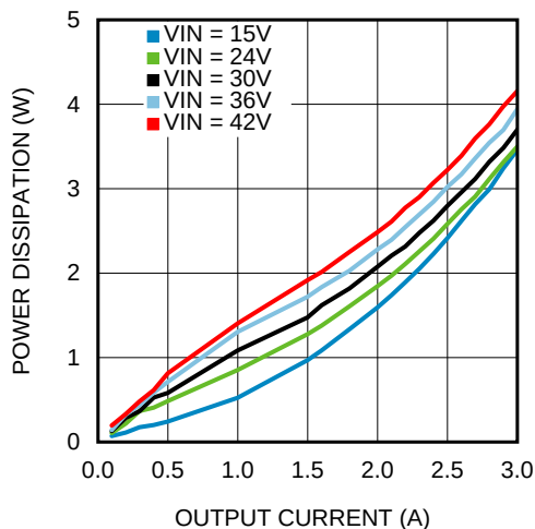
Figure 51. Power Dissipation V_{OUT} = 12V T_A = 85^\circ C
