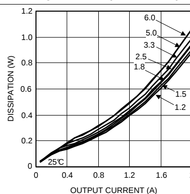
Figure 4. Dissipation 12-V Input
