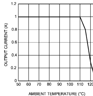
Thermal Derating Curve V_{IN} = 24\text{V} , V_{OUT} = 5.0\text{V} ,
