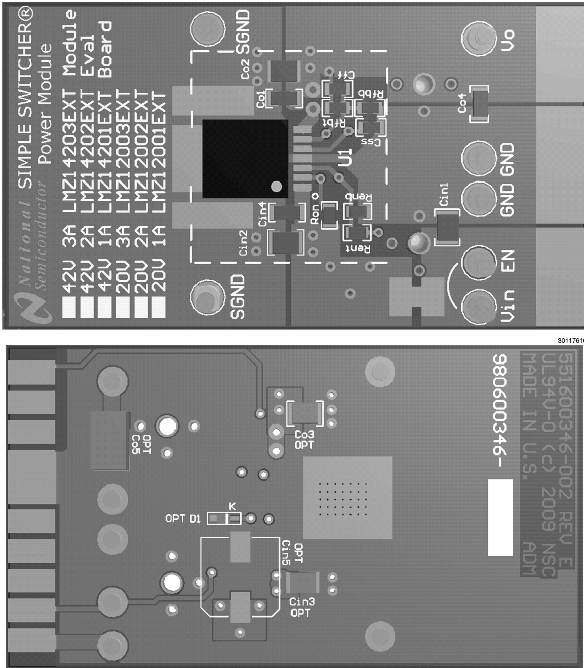
FIGURE 1. Top View and Bottom View of Evaluation PCB
