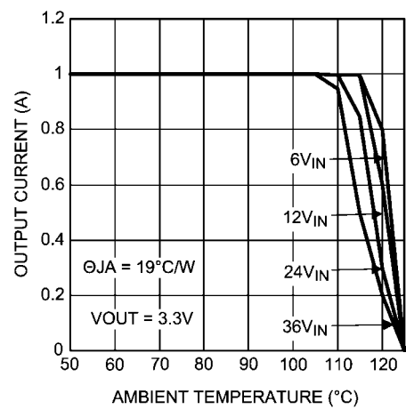
Thermal Derating V OUT = 3.3V
