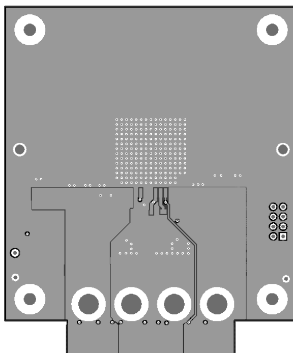
Figure 5. Top Layer
