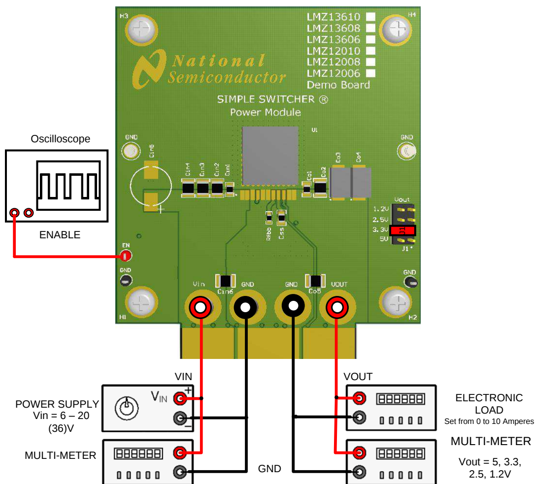
Figure 2. Board Connection Diagram
