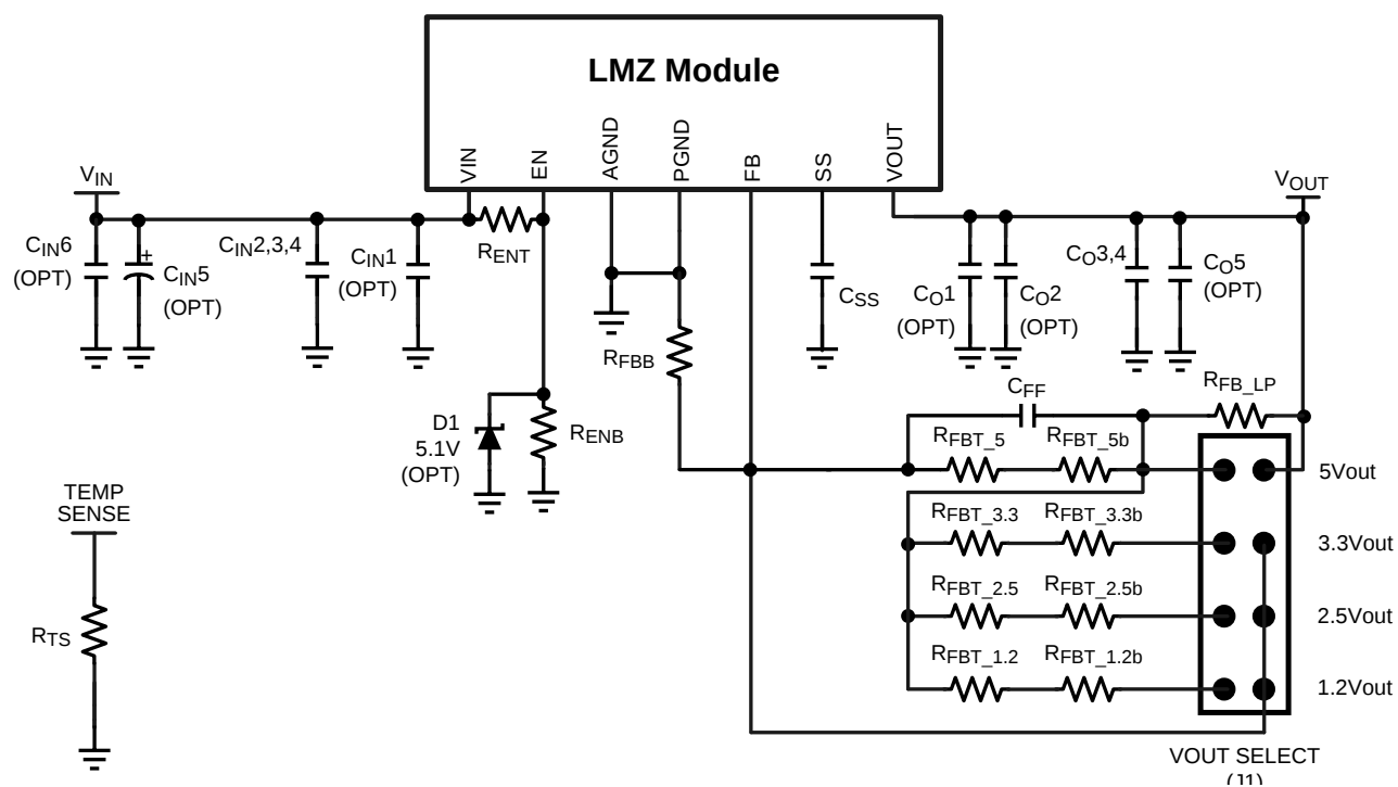
Figure 1. Simplified Schematic
