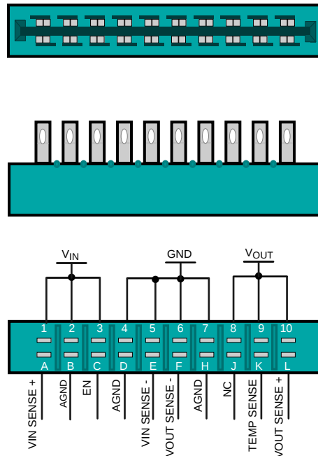
Figure 3. Edge Connector Diagram
