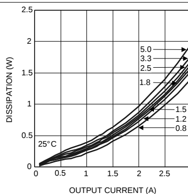
Figure 2. Dissipation 6-V Input at 25°C
