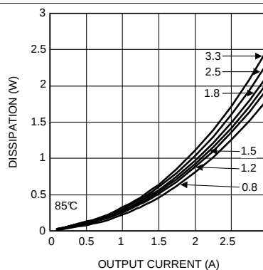
Figure 6. Dissipation 6-V Input at 85°C
