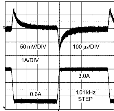
LMZ14203EXT Transient Response V_{IN} = 24V V_{OUT} = 3.3V , 0.6 A to 3A Step
