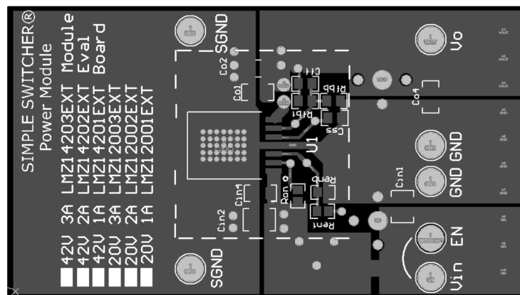
FIGURE 2. Top Layer
