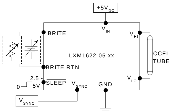
Figure 5 - Brightness Control
