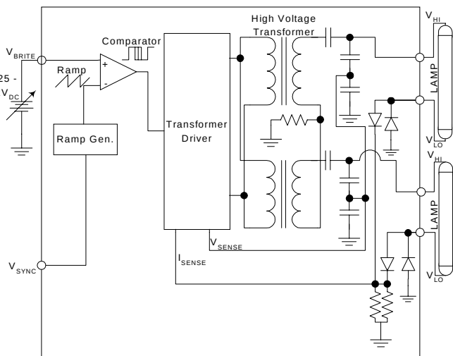
Figure 4 – RangeMAX Simplified Block Diagram
