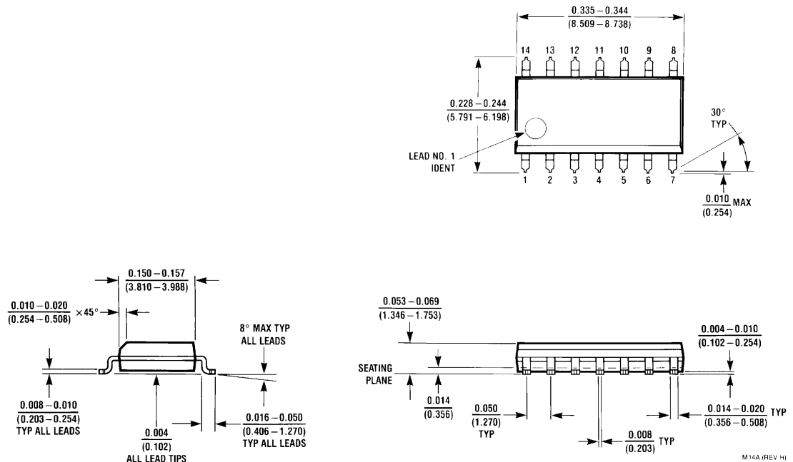
14-Pin Small Outline NS Package Number M14A
