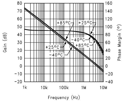
Gain and Phase Margin vs. Frequency (Temp. = 25, -40, 85^\circ C, R_L = 10k\Omega) 2.7V
