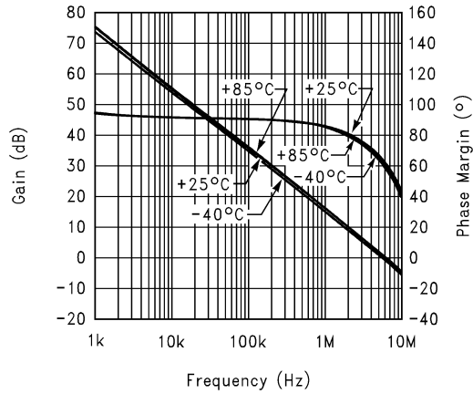
Gain and Phase Margin vs. Frequency (Temp. = 25, -40, 85^\circ C, R_L = 10k\Omega) 5V
