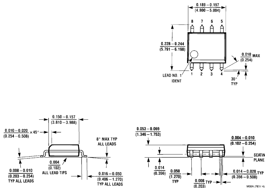
8-Pin Small Outline NS Package Number M08A
