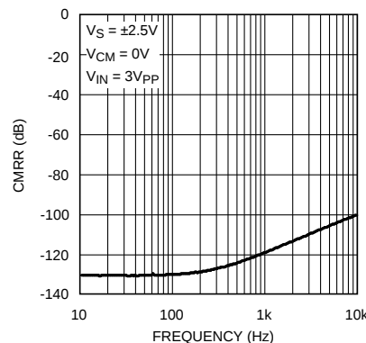
Figure 6. CMRR vs. Frequency
