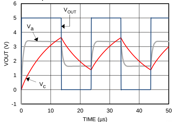
Figure 25. Square-Wave Oscillator Output Waveform
