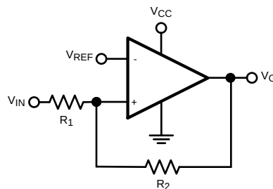
Figure 21. Basic Comparator With Hysteresis
