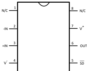
Pin Functions for SOIC (Single)
