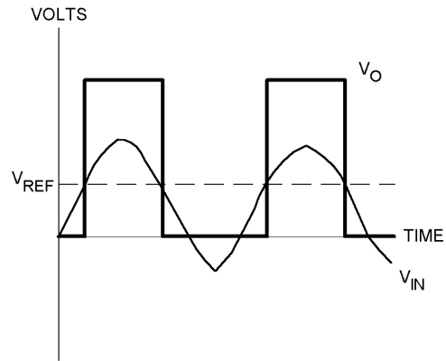
FIGURE 2. LMV7271 Basic Comparator
