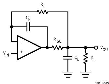
FIGURE 6. Indirectly Driving A Capacitive A Load with DC Accuracy
