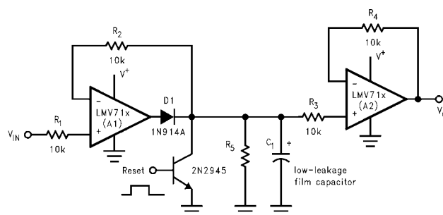
FIGURE 7. Peak Detector
