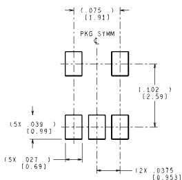
LAND PATTERN RECOMMENDATION
