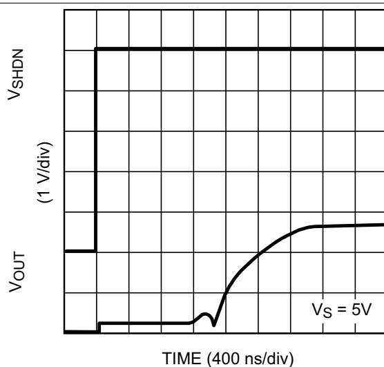
Figure 42. Turnon Time
