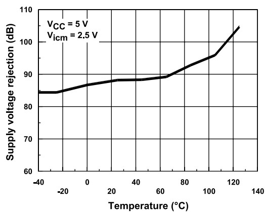
Figure 6. Supply voltage rejection vs. temperature ( V_{\text{CC}} = 5\text{ V} , V_{\text{icm}} = 2.5\text{ V} )
