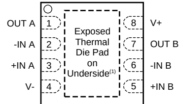
LMV358A DSG Package 8-Pin WSON With Exposed Thermal Pad Top View
