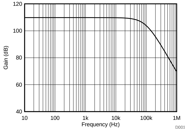
Figure 35. Photodiode Amplifier Circuit AC Gain Results
