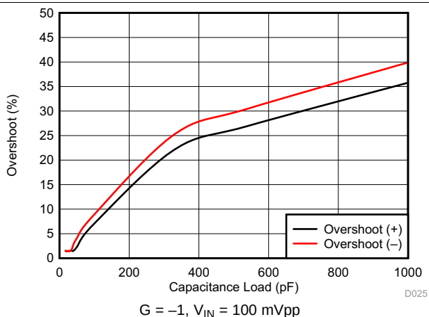
Figure 20. Small Signal Overshoot vs Capacitive Load
