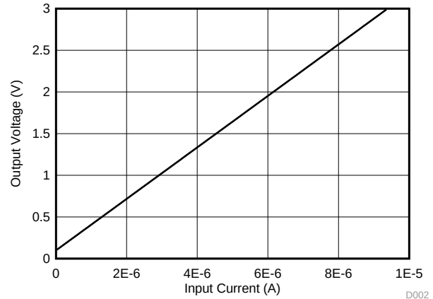
Figure 36. Photodiode Amplifier Circuit DC Results
