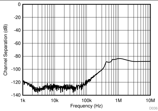
Figure 31. Channel Separation
