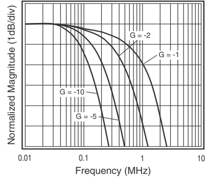
Inverting Frequency Response V_S = +5\text{V}
