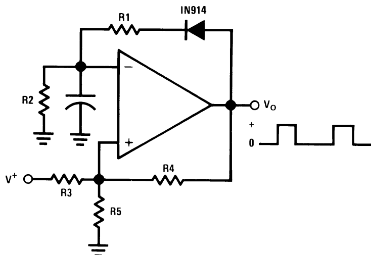
Figure 65. Pulse Generator
