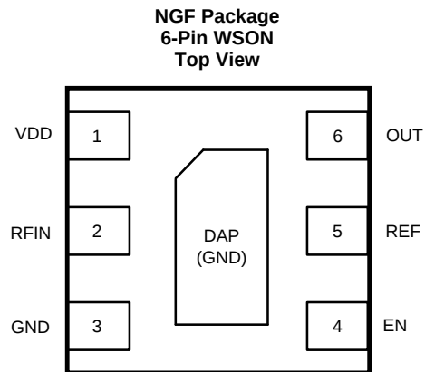
Pin Functions
