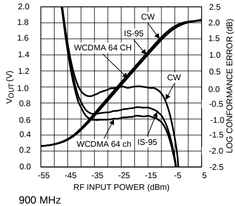
Figure 55. Output Voltage and Log Conformance Error vs RF Input Power for Various Modulation Types
