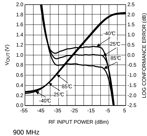
Figure 8. Mean Output Voltage and Log Conformance Error vs RF Input Power
