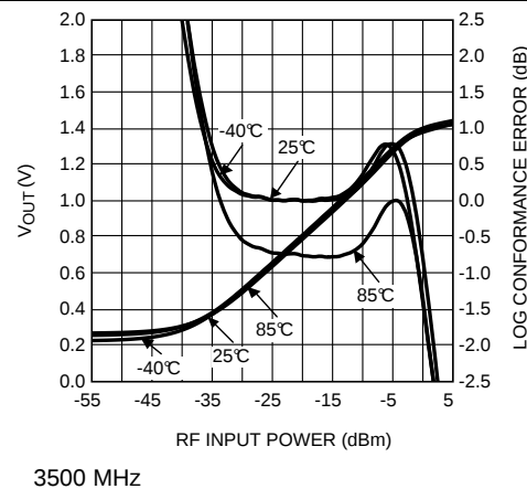
Figure 12. Mean Output Voltage and Log Conformance Error vs RF Input Power
