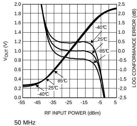
Figure 7. Mean Output Voltage and Log Conformance Error vs RF Input Power
