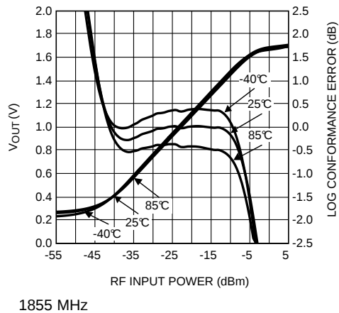
Figure 9. Mean Output Voltage and Log Conformance Error vs RF Input Power
