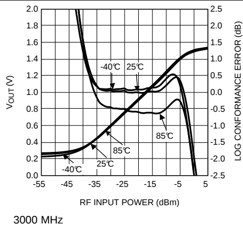
Figure 11. Mean Output Voltage and Log Conformance Error vs RF Input Power
