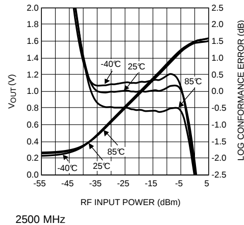
Figure 10. Mean Output Voltage and Log Conformance Error vs RF Input Power
