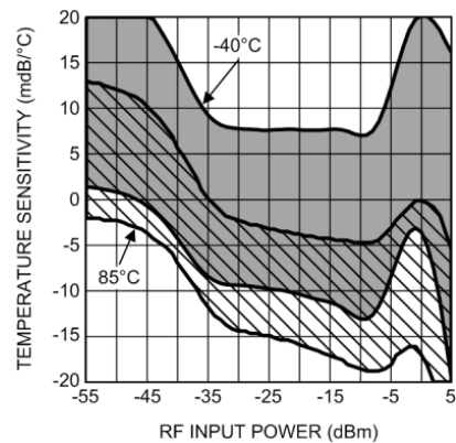
3000 MHz
