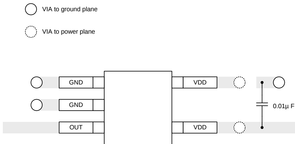
Figure 20. SC70 Package Recommended Layout
