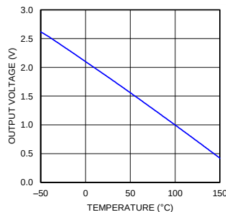
Figure 13. Analog Output Transfer Function
