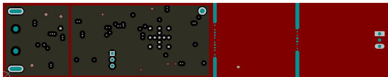
Figure 19. Power Layer Routing
