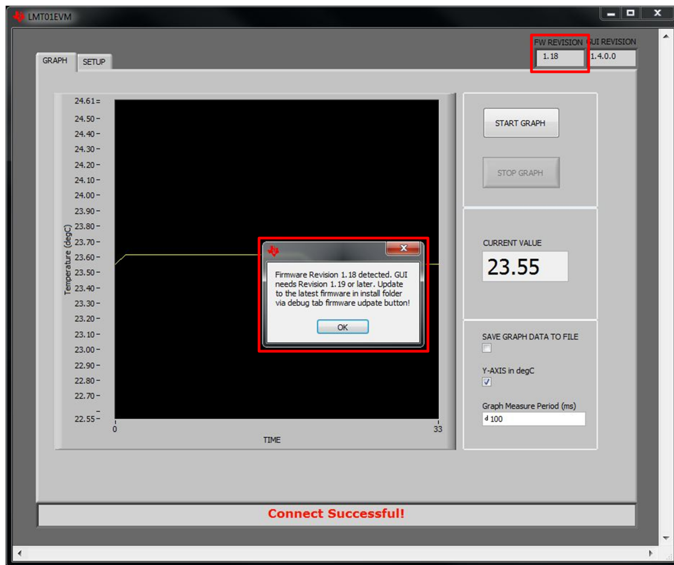
Figure 4. Firmware Revision Number
