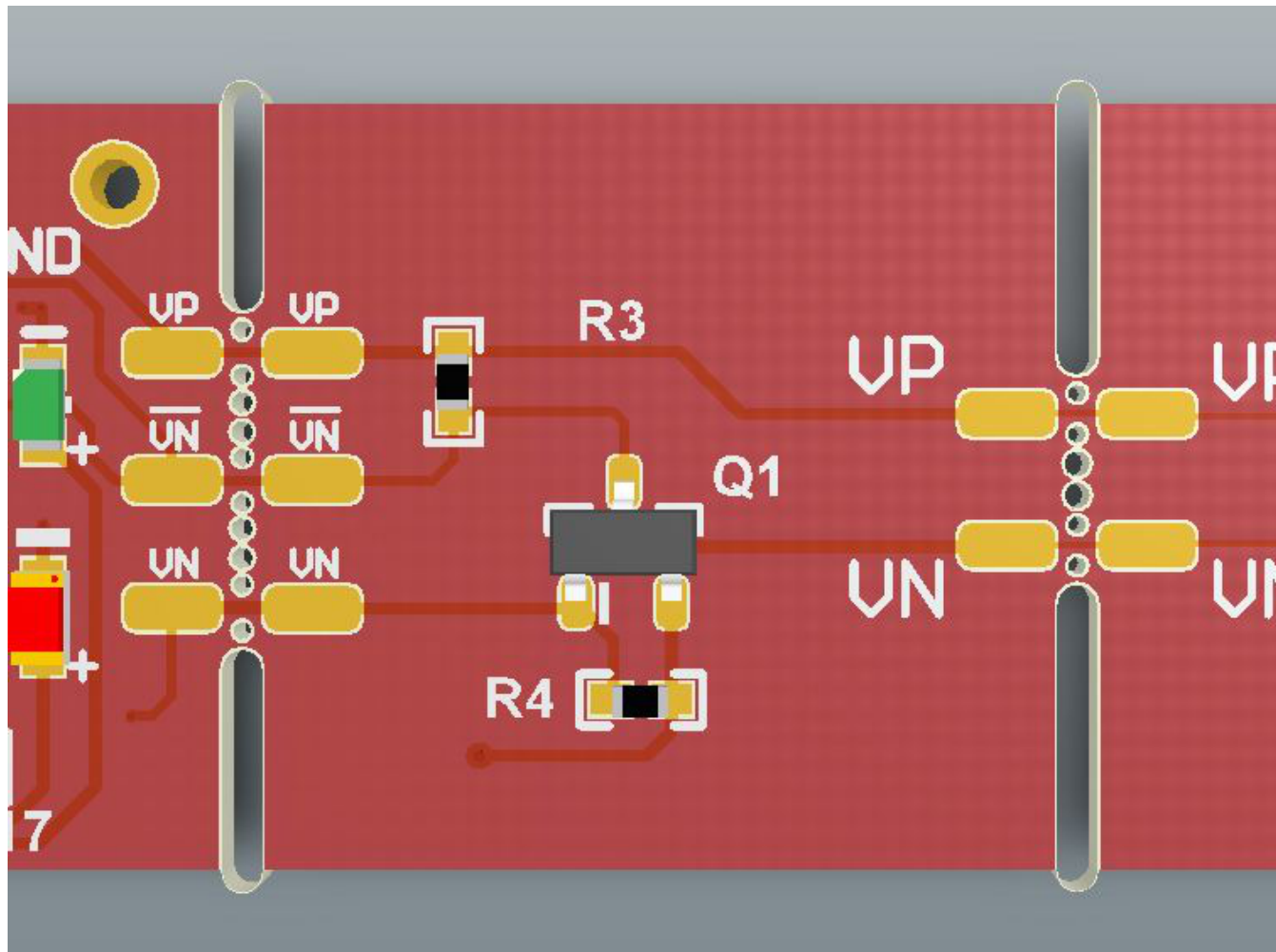
Figure 12. Breakout Slots and Exposed Pads
