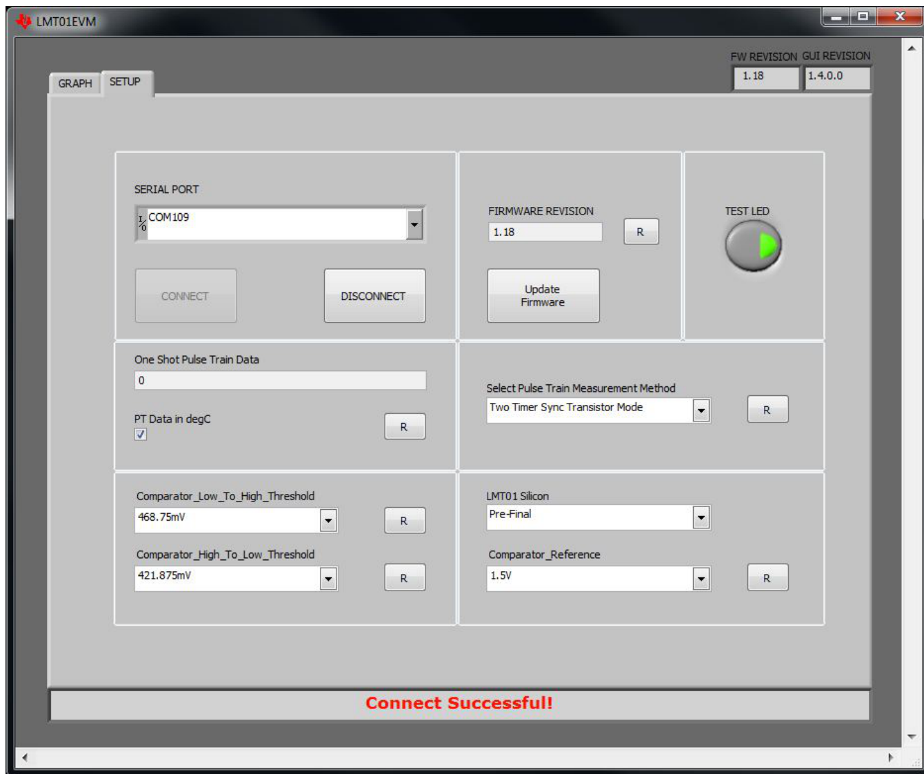
Figure 10. SETUP Tab page
