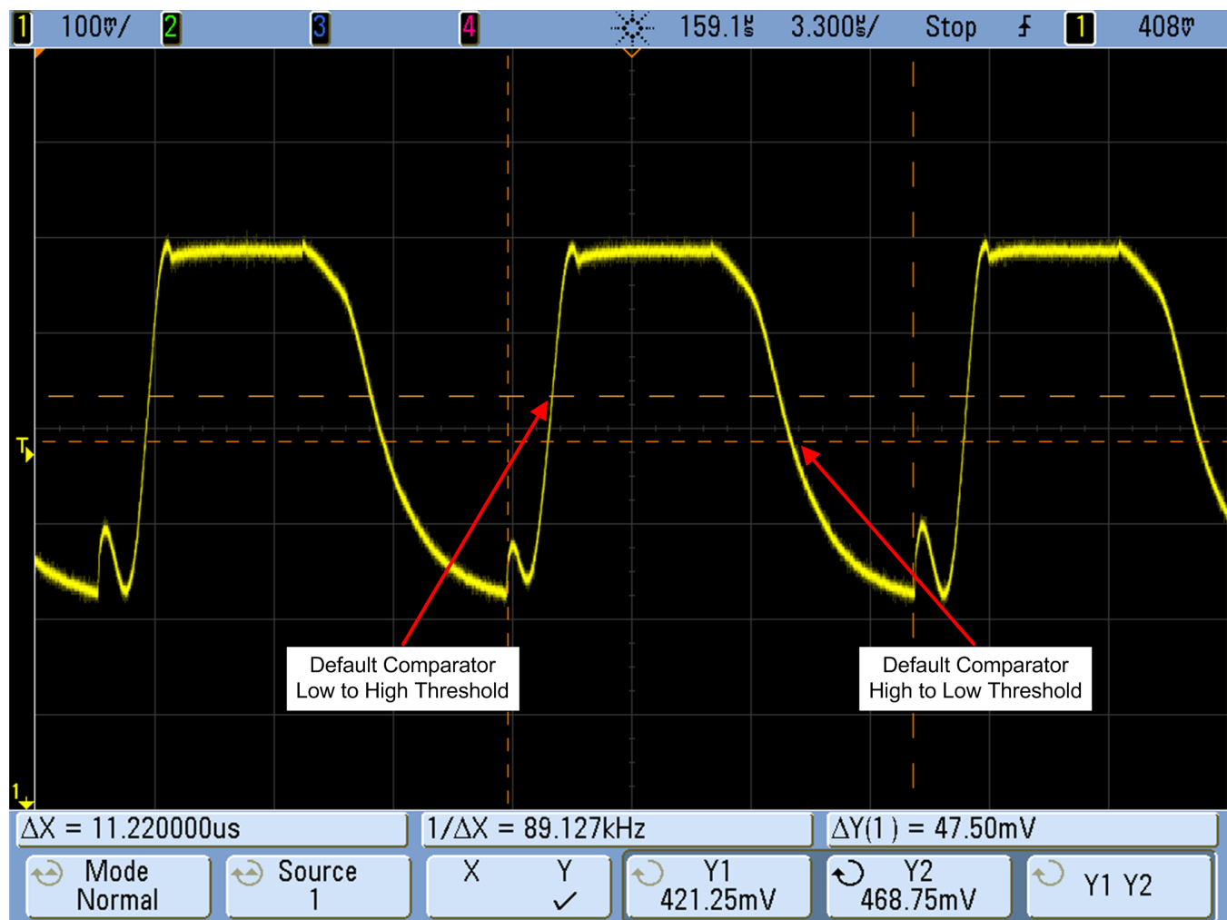
Figure 9. Comparator Threshold
