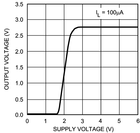
Dropout Characteristics
