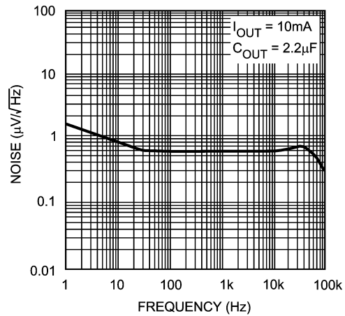
Noise Characteristics
