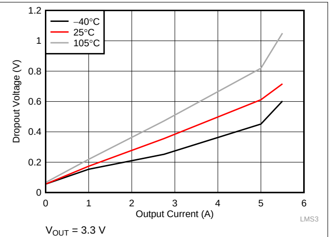
Figure 43. Dropout for ≥ 330 kHz
