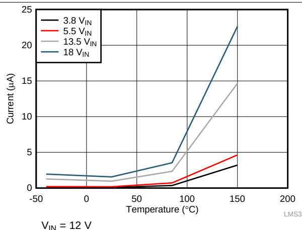
Figure 6. Shutdown Current
