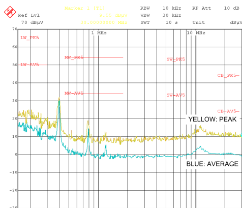
LMS3655-Q1 Conducted EMI: \text{V}_{\text{OUT}} = 5\text{ V} , \text{I}_{\text{OUT}} = 5\text{ A}
