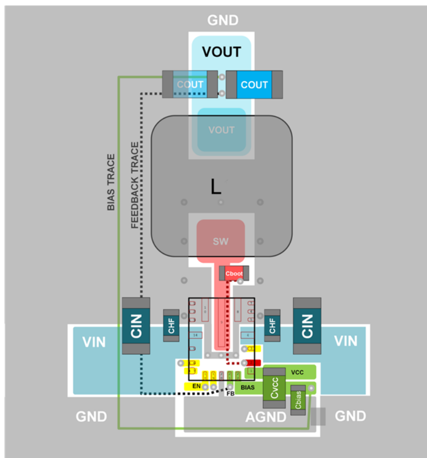
Figure 54. Recommended Layout for LMS36x5-Q1
