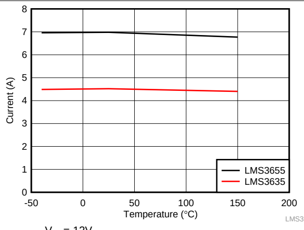
Figure 4. Low-Side/Valley Current Limit for LMS36x5-Q1
