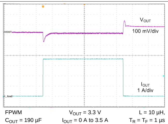
Figure 47. Load Transient
