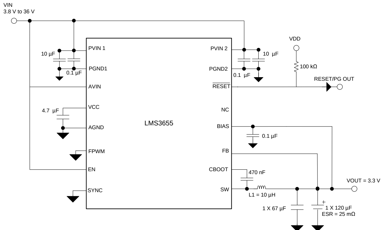
Figure 35. Fixed 3.3-V, 5.5-A Output Power Supply
