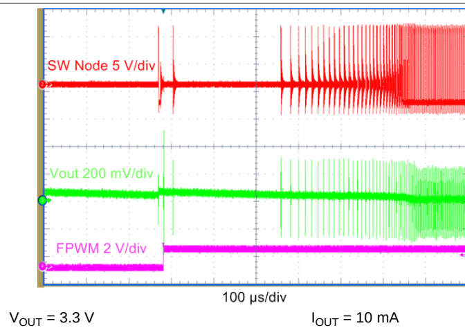
Figure 48. Mode Change Transient AUTO to FPWM mode
