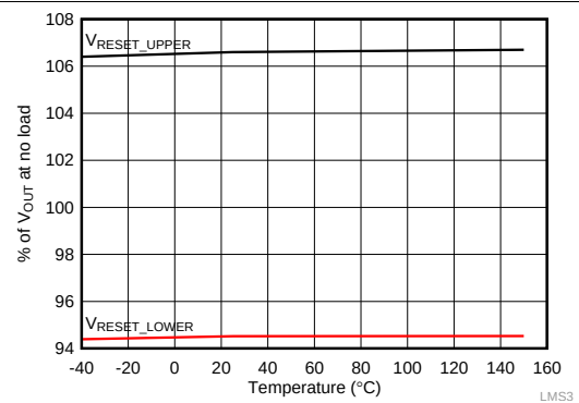
Figure 8. RESET Threshold as Percentage of Output Voltage
