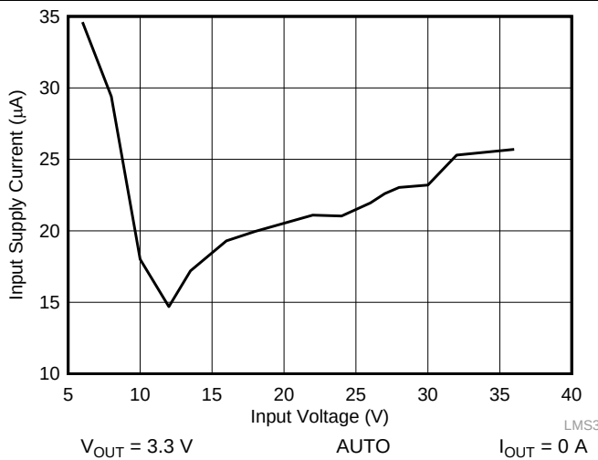
Figure 40. Input Supply Current (Includes Leakage Current of Capacitor)
