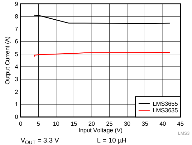
Figure 45. Output Current Level for Overcurrent Protection Trip
