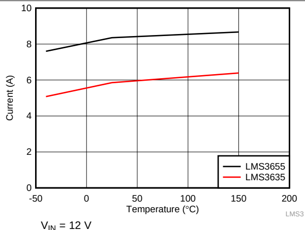
Figure 3. High-Side/Peak Current Limit for LMS36x5-Q1
