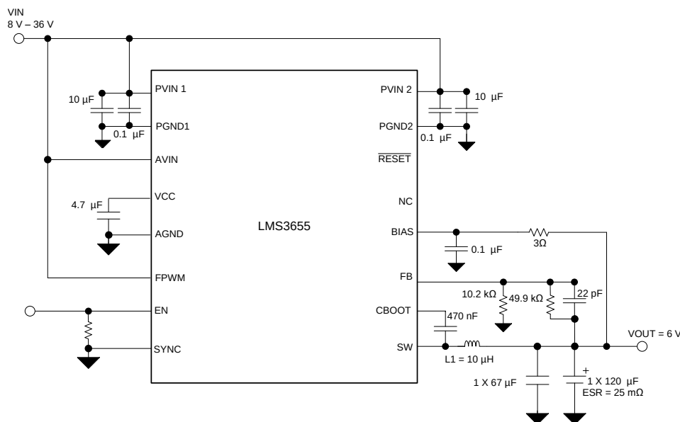
Figure 49. 6-V Output Power Supply
