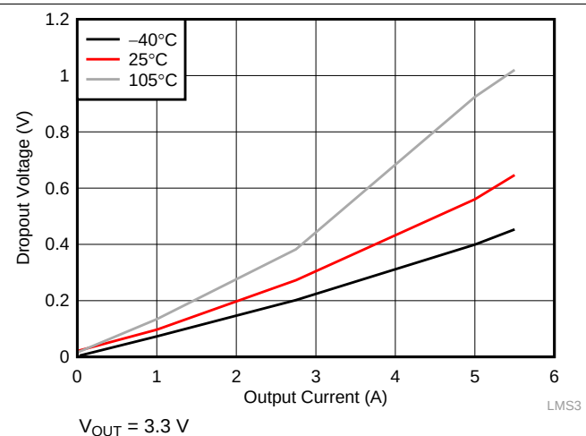
Figure 42. Dropout for -3% Regulation
