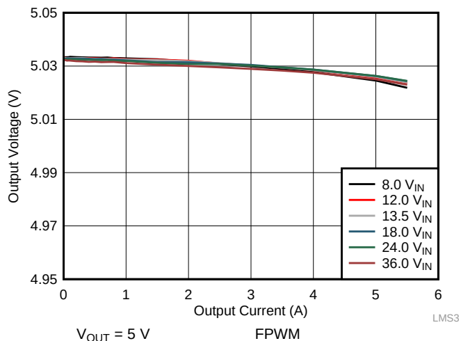
Figure 27. Load and Line Regulation
