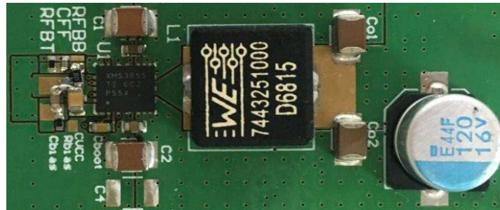
Figure 55. LMS3655MQEVM Layout
