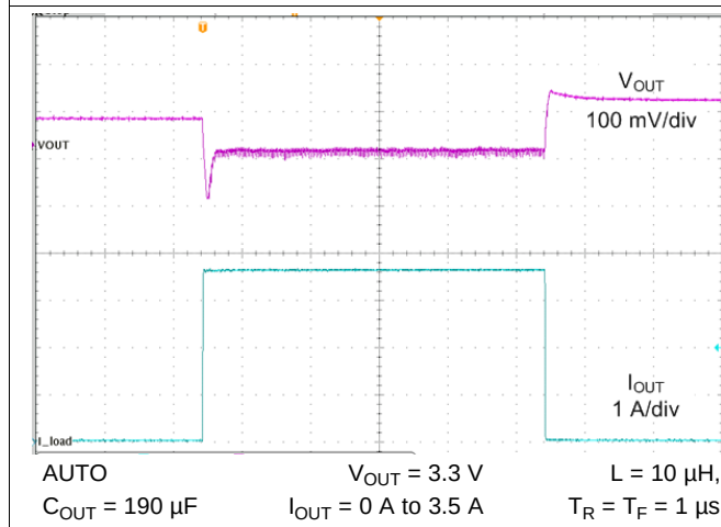
Figure 46. Load Transient
