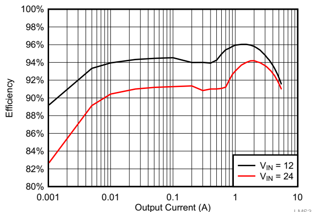
LMS3655-Q1 Efficiency: \text{V}_{\text{OUT}} = 5\text{ V}
