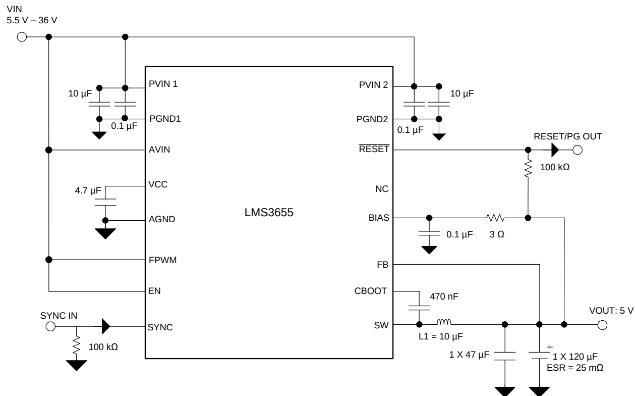
Figure 23. Fixed 5-V, 5.5-A Output Power Supply
