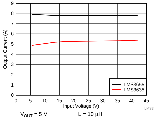
Figure 32. Output Current Level Limit Before Overcurrent Protection
