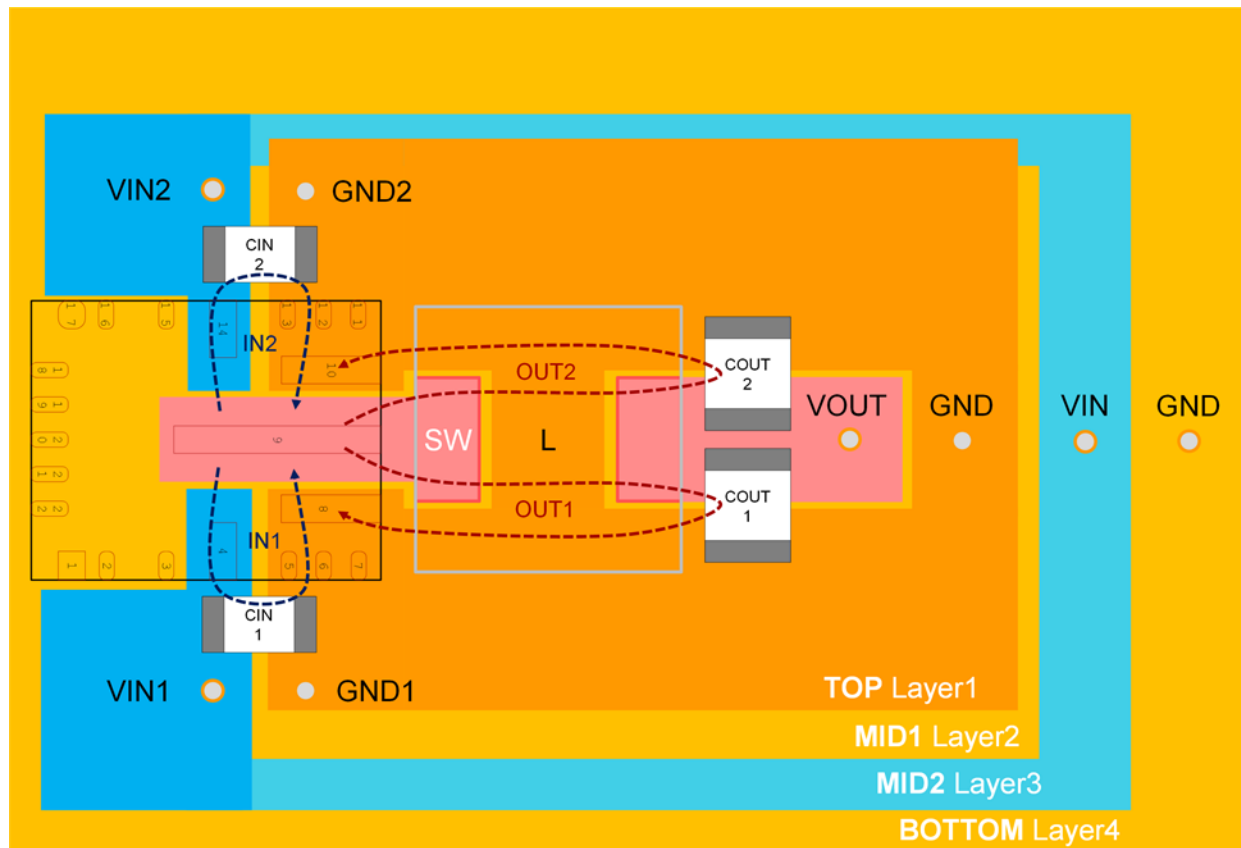
Figure 53. Layout of the Power Components and Current Flow
