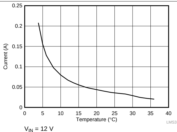
Figure 5. Short Circuit Average Input Current for LMS3635-Q1
