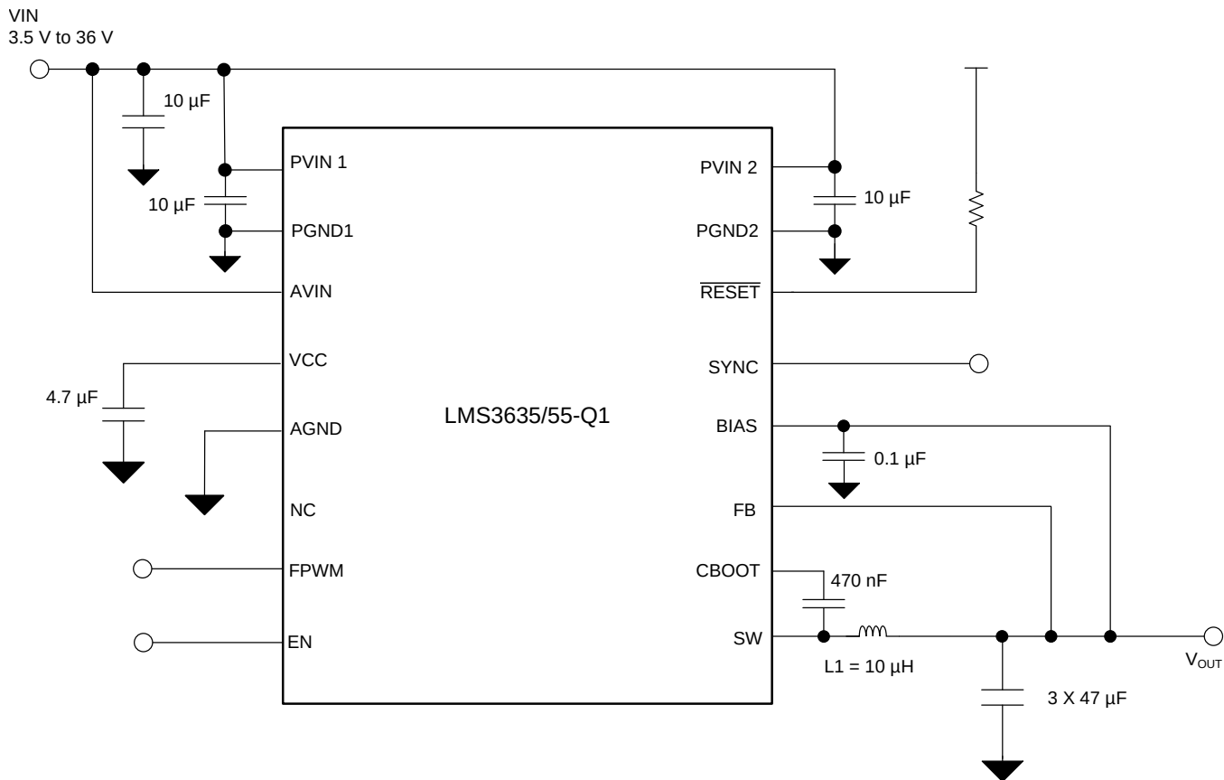
Figure 20. General Application Circuit
