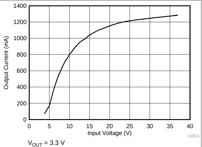
Figure 41. Load Current for PFM-to-PWM Transition
