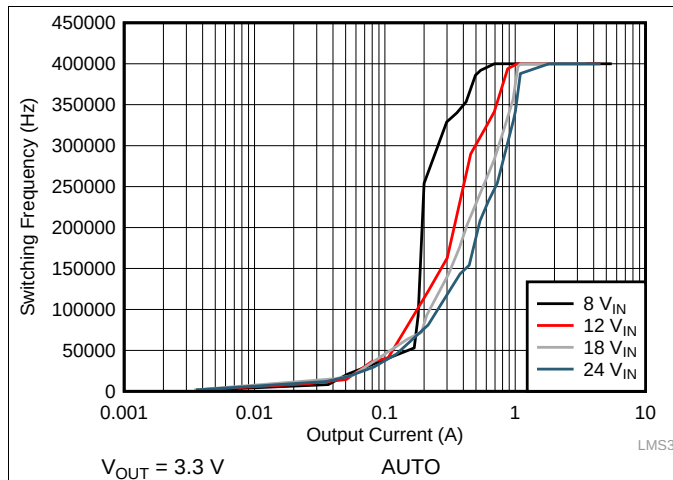
Figure 44. Switching Frequency vs Load Current
