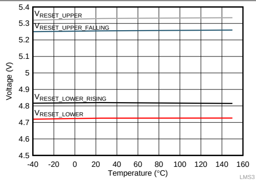
Figure 7. RESET Threshold Fixed 5-V Output
