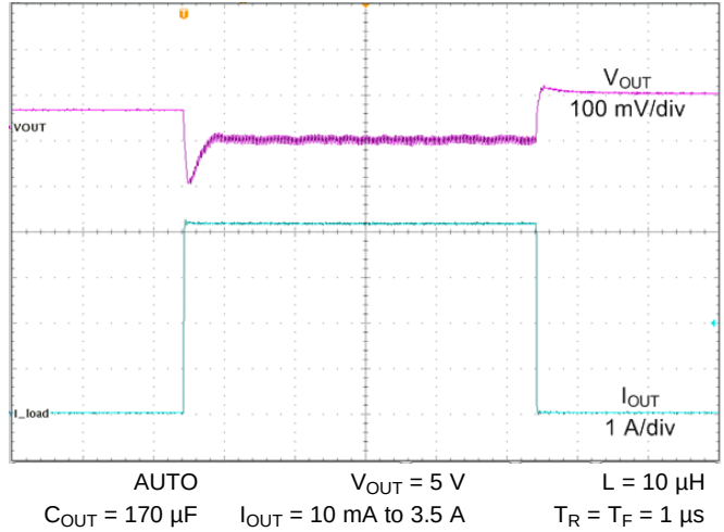
Figure 33. Load Transients
