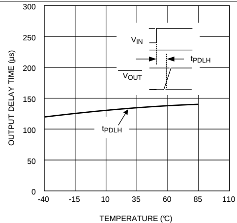
Figure 4. Propagation Delay Time ( t_{PDL} ) vs Temperature
