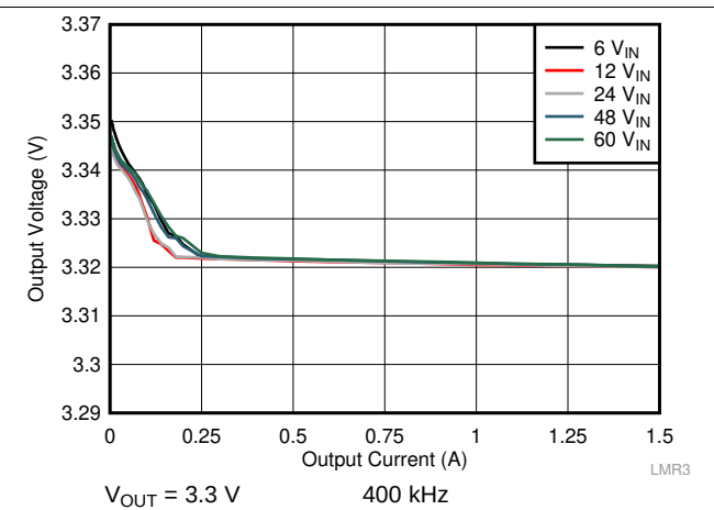
Figure 25. Load Regulation
