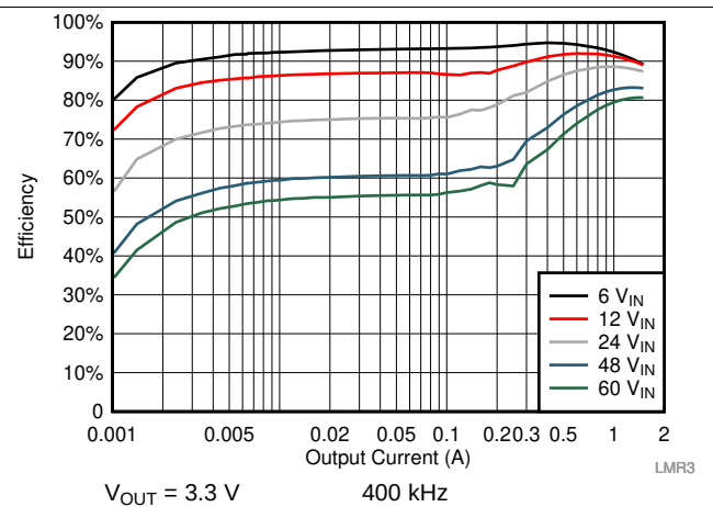
Figure 23. Efficiency
