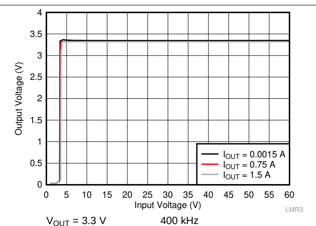
Figure 27. Line Regulation
