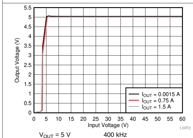
Figure 26. Line Regulation
