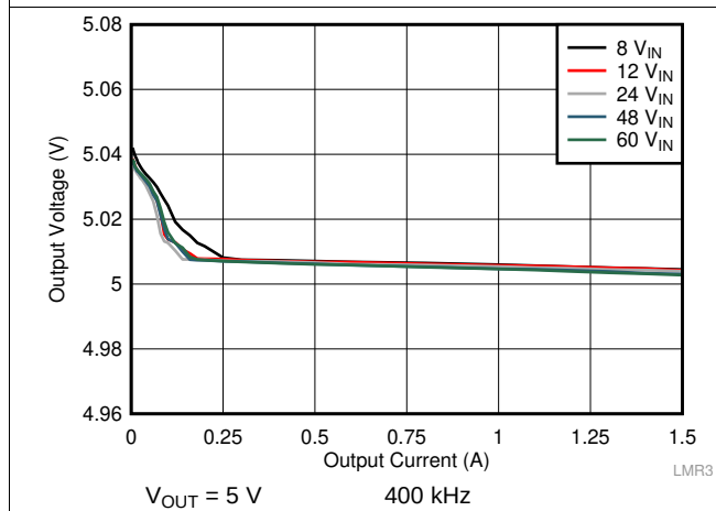
Figure 24. Load Regulation
