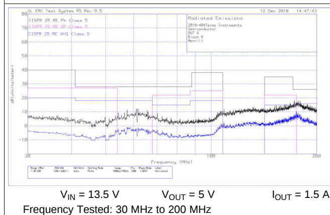
Figure 38. Radiated EMI Bicon Horizontal vs. CISPR25 Limits
