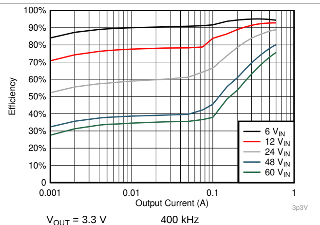
Figure 23. Efficiency
