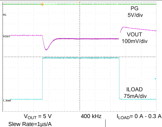
Figure 32. Load Transient
