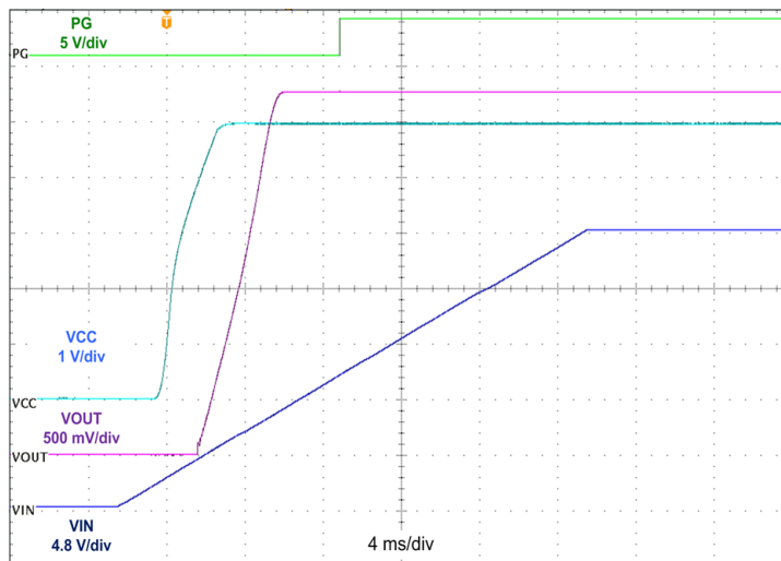
Figure 11. Typical Start-up Behavior V_{IN} = 24\text{ V} , V_{OUT} = 3.3\text{ V} , I_{OUT} = 0.6\text{ A}
