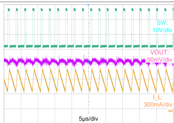
Figure 14. Typical PWM Switching Waveforms V_{IN} = 24\text{ V} , V_{OUT} = 5\text{ V} , I_{OUT} = 600\text{ mA} , f_S = 400\text{ kHz}
