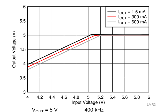
Figure 26. Overall Dropout Characteristic
