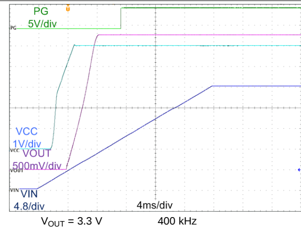
Figure 31. Start-Up Waveform
