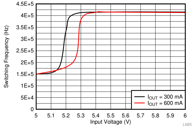
Figure 16. Typical f_{SW} vs Output Current f_{SW} = 400\text{ kHz}
