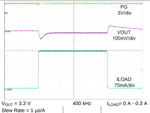
Figure 33. Load Transient
