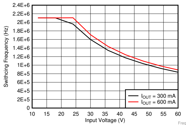
Figure 17. Switching Frequency vs Input Voltage V_{OUT} = 3.3\text{ V}
