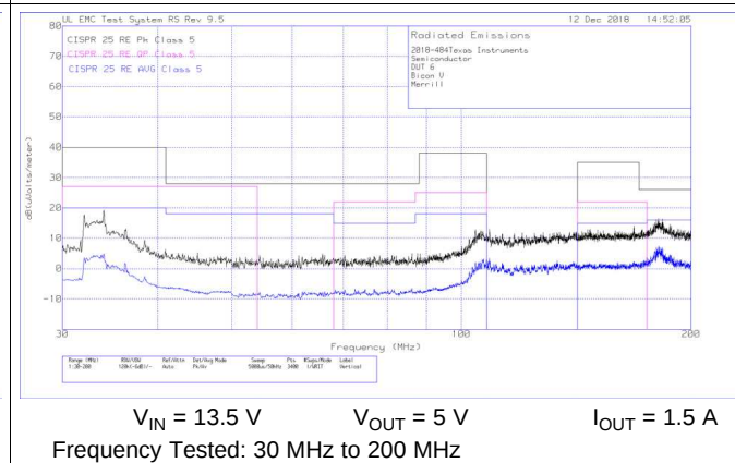
Figure 37. Radiated EMI Bicon Vertical vs. CISPR25 Limits
