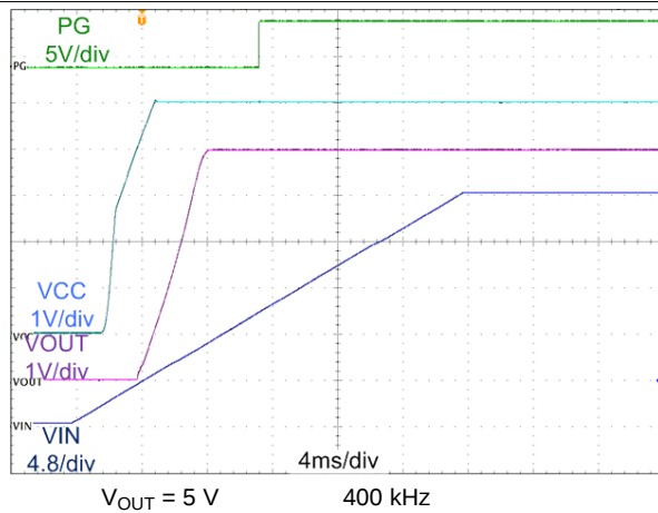
Figure 30. Start-Up Waveform
