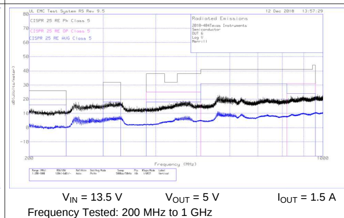
Figure 39. Radiated EMI Log Vertical vs. CISPR25 Limits
