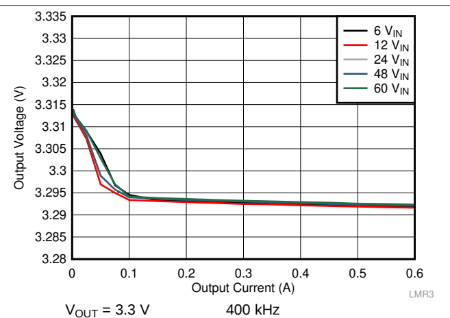
Figure 25. Load Regulation
