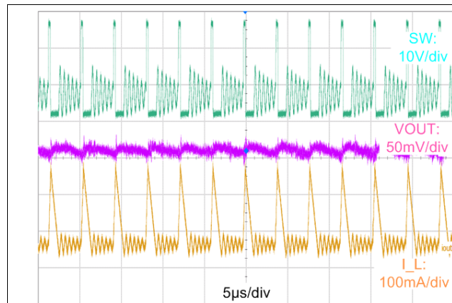
Figure 13. Typical PFM Switching Waveforms V_{IN} = 24\text{ V} , V_{OUT} = 5\text{ V} , I_{OUT} = 30\text{ mA}
