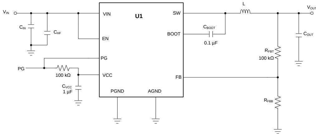
Figure 48. Circuit for Application Curves
