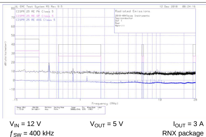
Figure 47. Radiated EMI Rod Antenna
