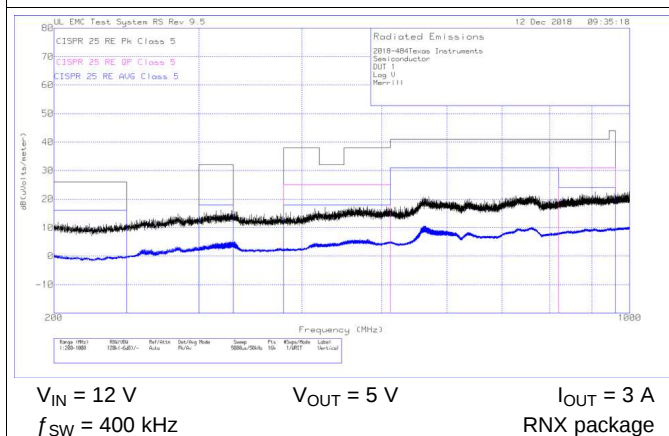
Figure 46. Radiated EMI Log-periodic Antenna (Vertical)
