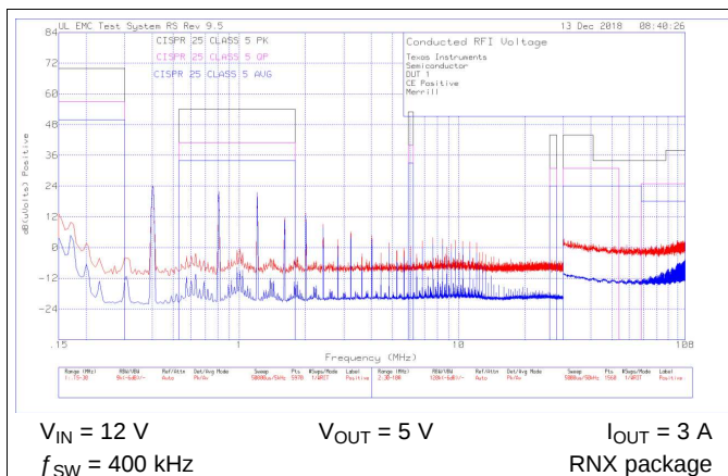
Figure 42. Conducted EMI
