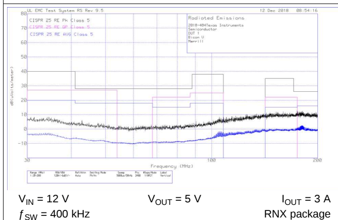
Figure 44. Radiated EMI Biconical Antenna (Vertical)
