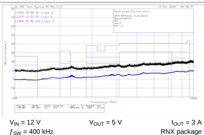
Figure 45. Radiated EMI Log-periodic Antenna (Horizontal)
