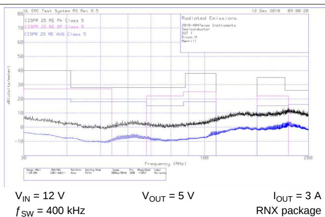
Figure 43. Radiated EMI Biconical Antenna (Horizontal)
