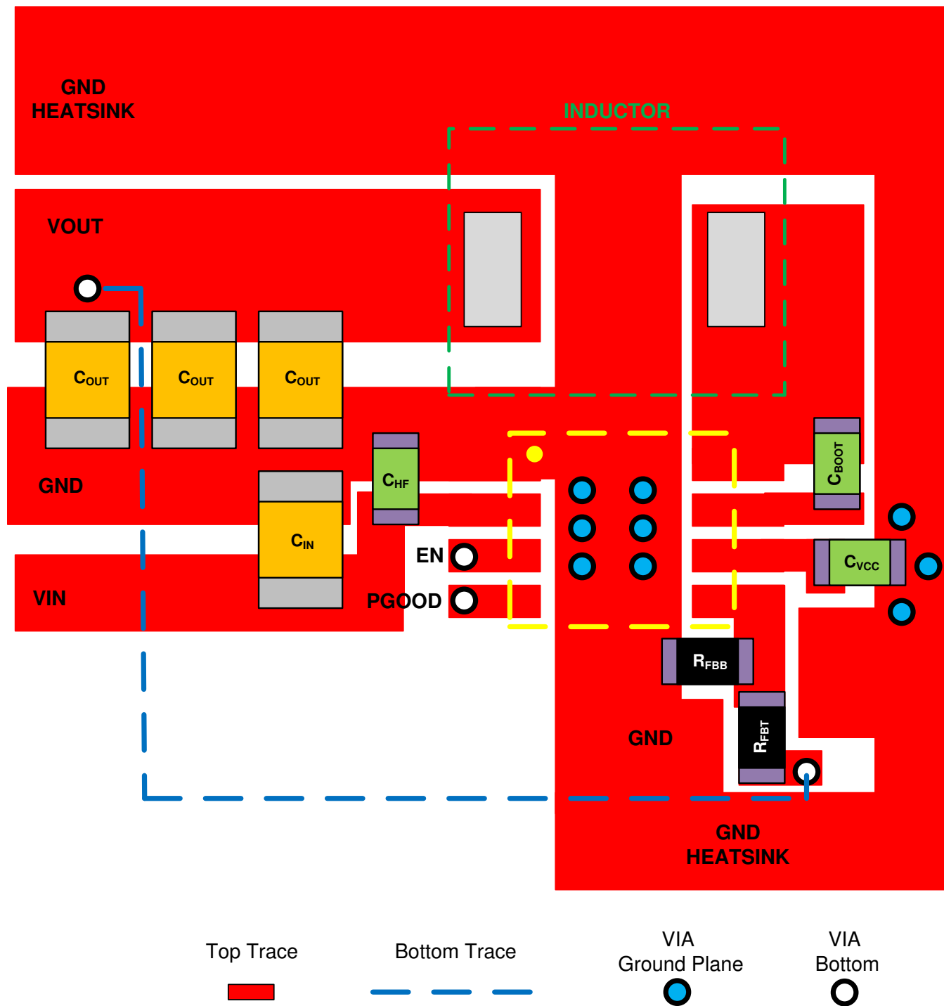
Figure 53. Example Layout for WQFN Package
