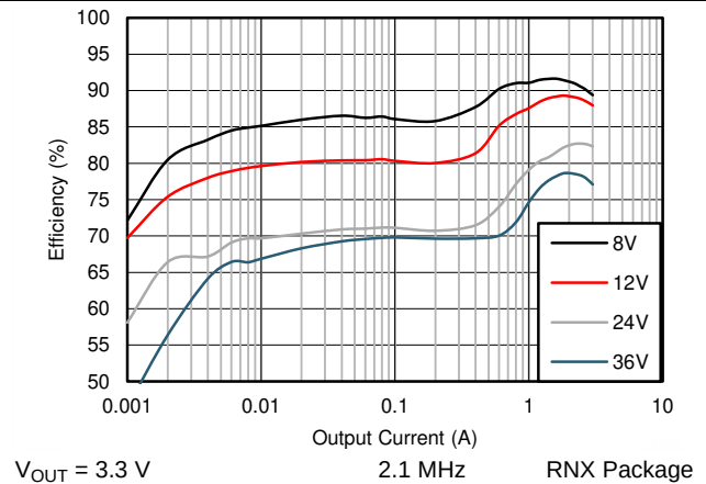
Figure 37. Efficiency
