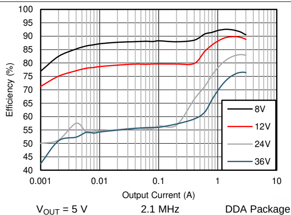
Figure 30. Efficiency
