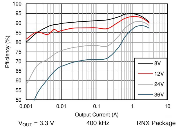
Figure 33. Efficiency
