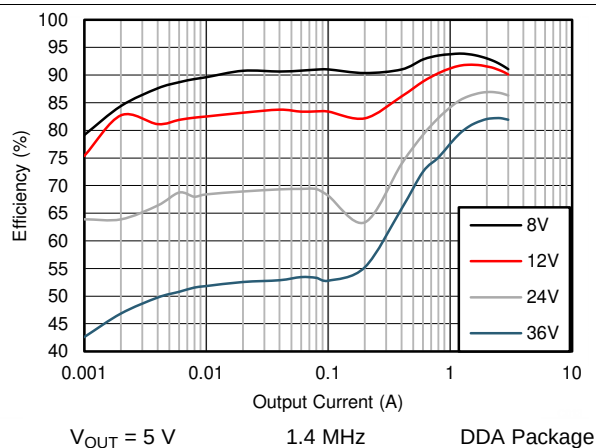
Figure 28. Efficiency
