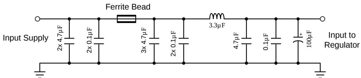
Figure 53. Typical Input EMI Filter Filter used only for EMI measurements found in Application Curves
