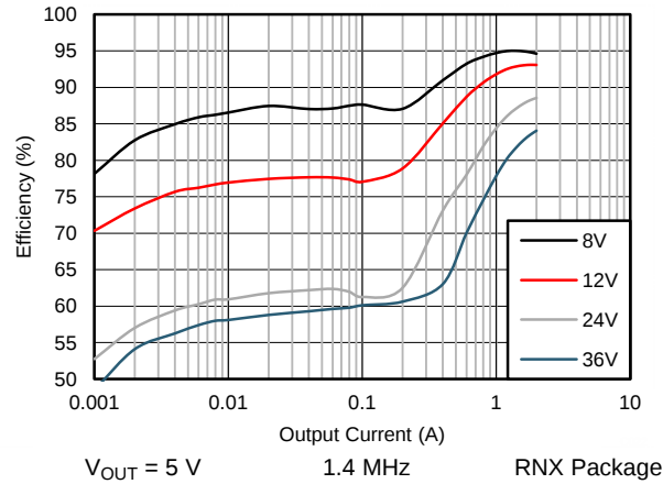
Figure 30. Efficiency
