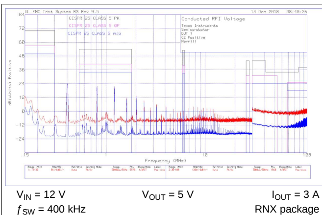
Figure 46. Conducted EMI
