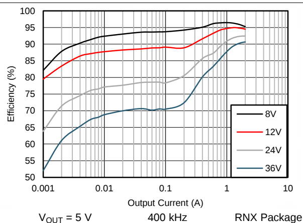
Figure 28. Efficiency
