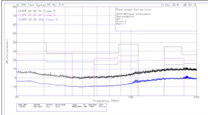
Figure 48. Radiated EMI Biconical Antenna (Vertical)
