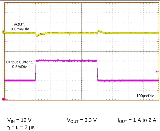
Figure 45. Load Transient
