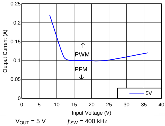
Figure 36. Mode Change Thresholds
