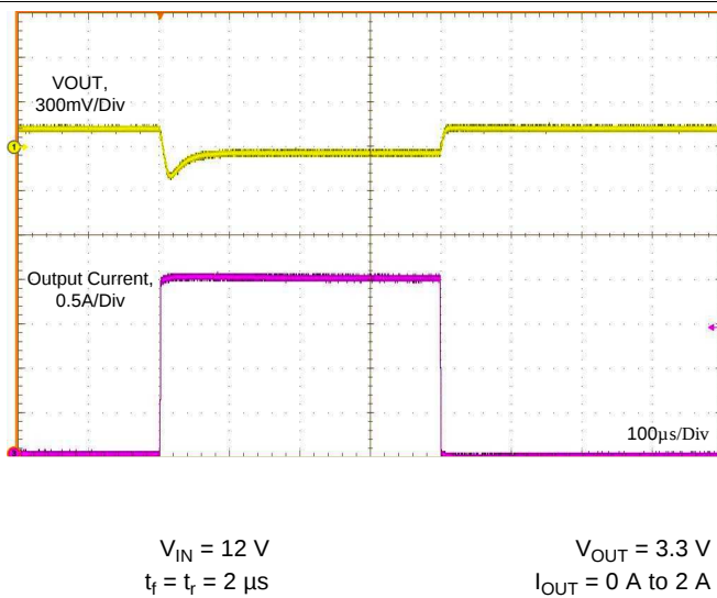
Figure 44. Load Transient
