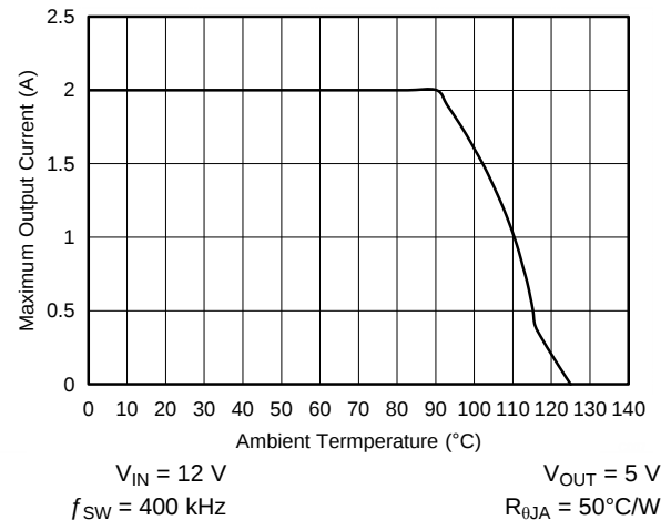
Figure 27. Maximum Output Current vs Ambient Temperature
