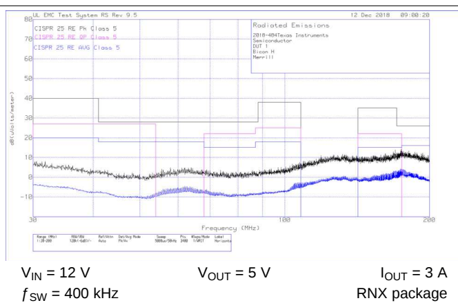
Figure 47. Radiated EMI Biconical Antenna (Horizontal)
