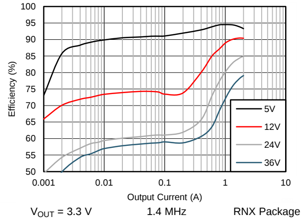
Figure 31. Efficiency
