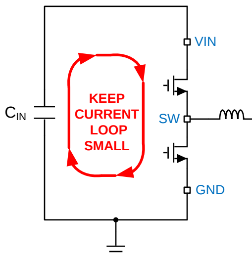
Figure 54. Current Loops with Fast Edges
