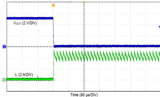
Figure 29. Output Short
