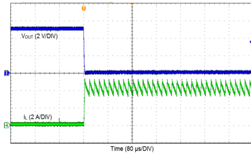
Figure 29. Output Short
