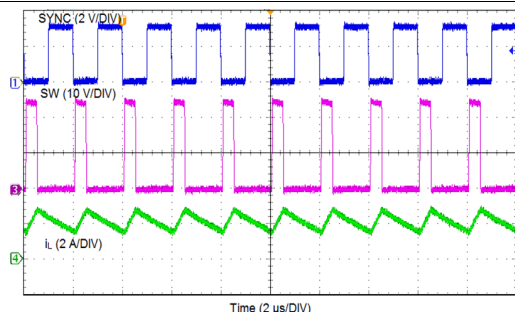
Figure 18. Synchronizing in CCM
