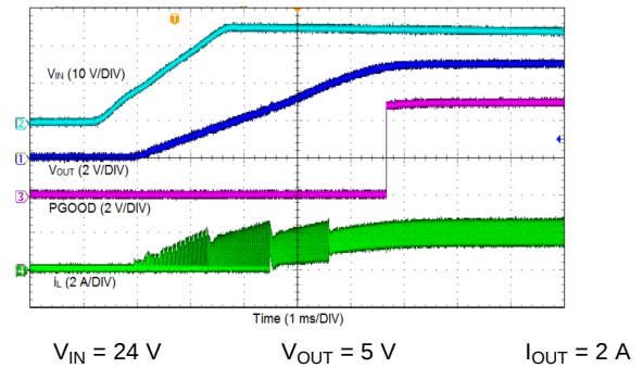
Figure 24. Start-up By V_{IN}
