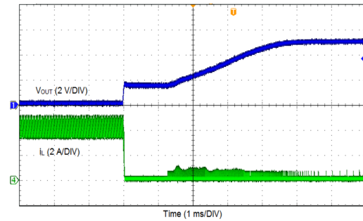
Figure 30. Output Short Recovery
