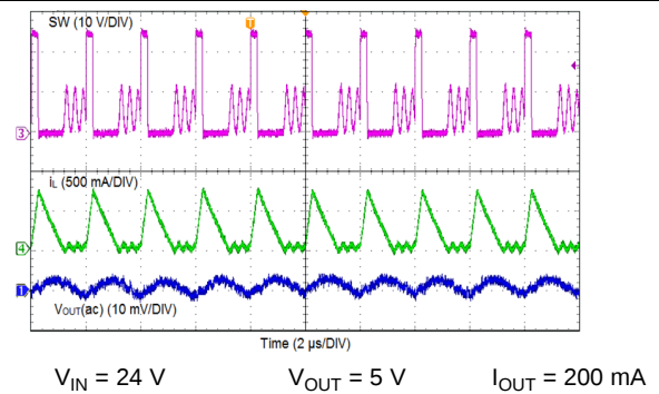
Figure 26. DCM Mode
