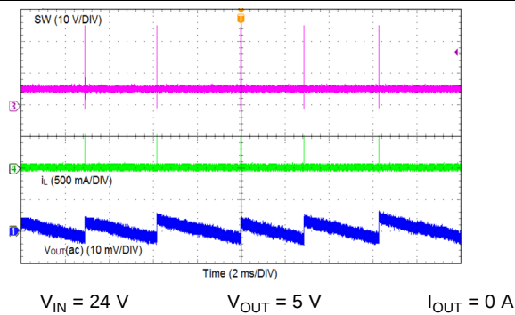
Figure 25. Sleep-mode
