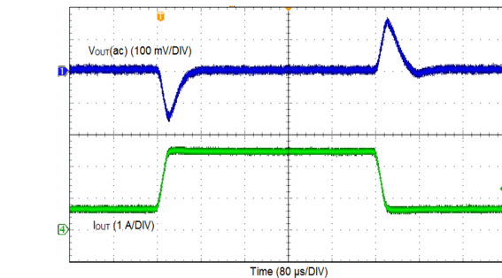
Figure 26. DCM Mode
