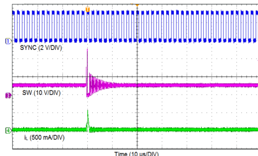
Figure 20. Synchronizing in Sleep-mode Mode
