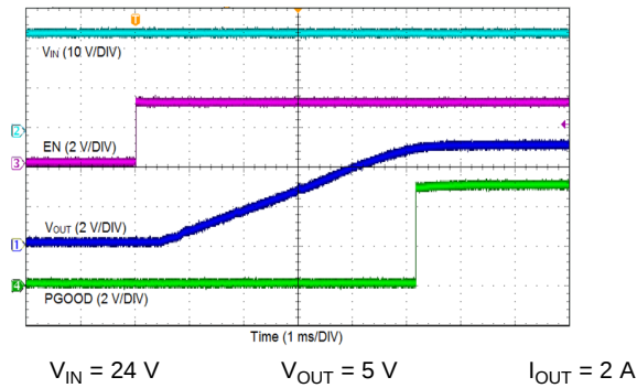
Figure 23. Start-up By EN
