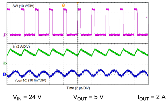
Figure 27. CCM Mode
