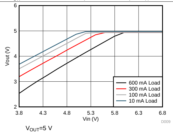
Figure 8. Dropout Curve
