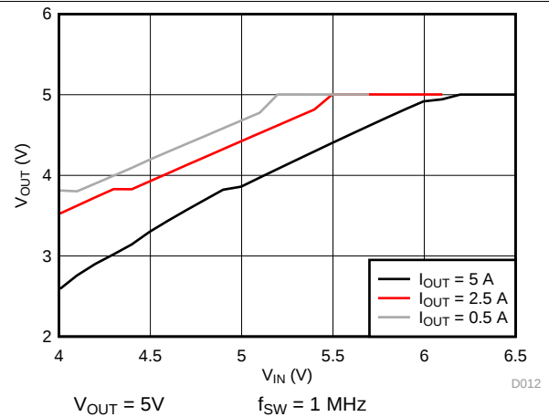
Figure 8. Dropout Curve
