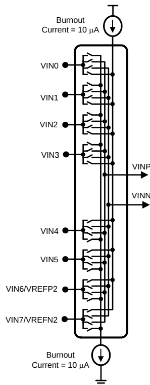
Figure 44. Burnout Currents
