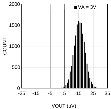
Figure 18. Histogram Without Calibration at Gain = 8
