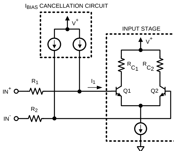
Figure 44. Input Bias Current Cancellation
