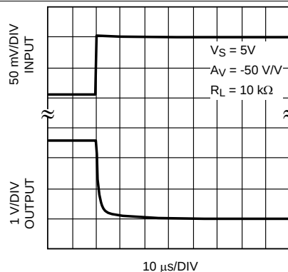
Figure 28. Overload Recovery Time
