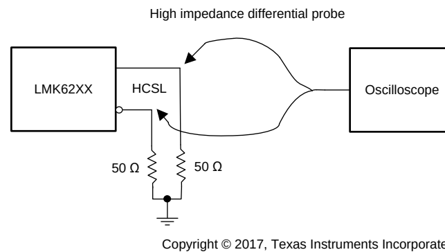
Figure 3. HCSL Output DC Configuration During Device Test (1)
