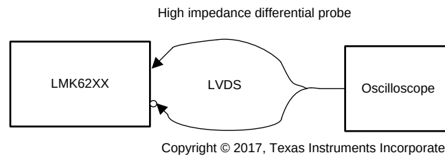
Figure 2. LVDS Output DC Configuration During Device Test
