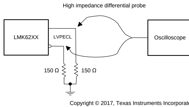
Figure 1. LVPECL Output DC Configuration During Device Test
