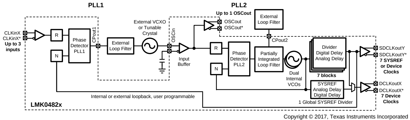
Figure 14. Simplified Functional Block Diagram for Nested 0-delay Dual Loop Mode
