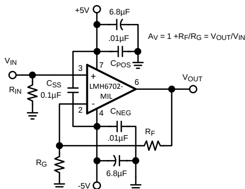
Figure 24. Recommended Non-Inverting Gain Circuit
