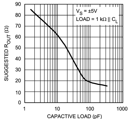
FIGURE 7. Suggested R_{\text{OUT}} vs. Capacitive Load
