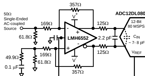
Figure 47. Split Supply
