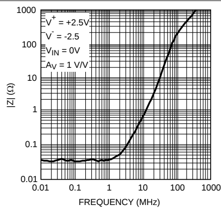
Figure 24. Closed Loop Output Impedance
