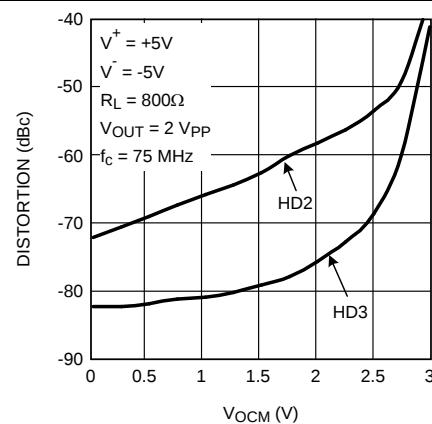
Figure 18. Distortion vs Output Common Mode Voltage
