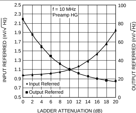
Figure 17. Noise vs Ladder Attenuation
