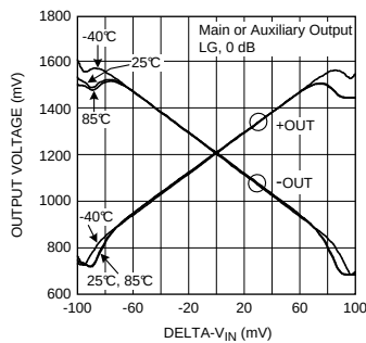
Figure 51. Output vs Input
