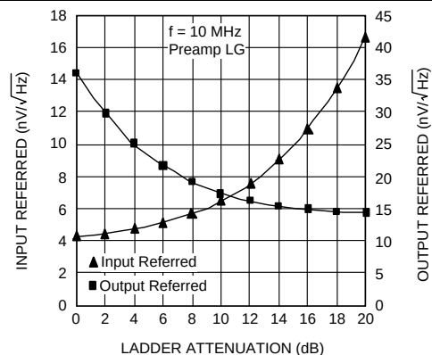
Figure 18. Noise vs Ladder Attenuation
