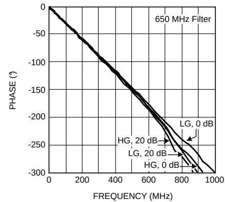
Figure 14. Phase vs Gain
