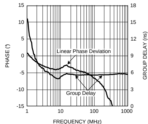
Figure 16. Linear Phase Deviation and Group Delay
