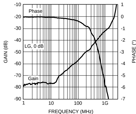
Figure 15. Balance Error
