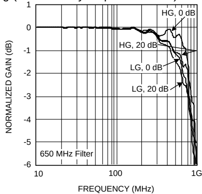
Figure 13. Response vs Gain
