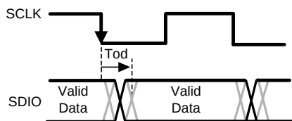
Figure 56. Read Timing
