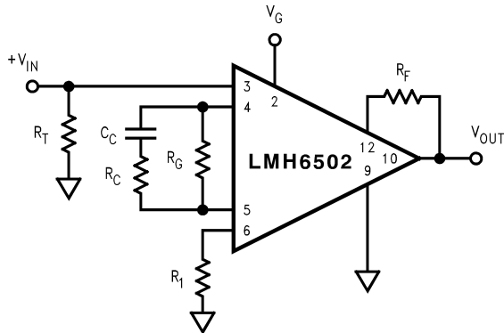
Figure 64. Frequency Shaping
